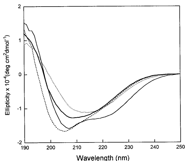
FIGURE 7 Unsmoothed circular dichroism spectra of SC3. SC3 in the monomeric form (thick line), SC3 after assembly at the water-air interface by shaking (dotted line), assembled SC3 dissolved in 25% TFE (dashed line), and SC3 assembled on a hydrophobic colloidal Teflon surface (thin line). Spectra are the average of 10 scans corrected by using a reference solution without the protein. Typically, a protein concentration of 3.5 \mu M in 20 mM phosphate buffer at pH 7.0 was used.
