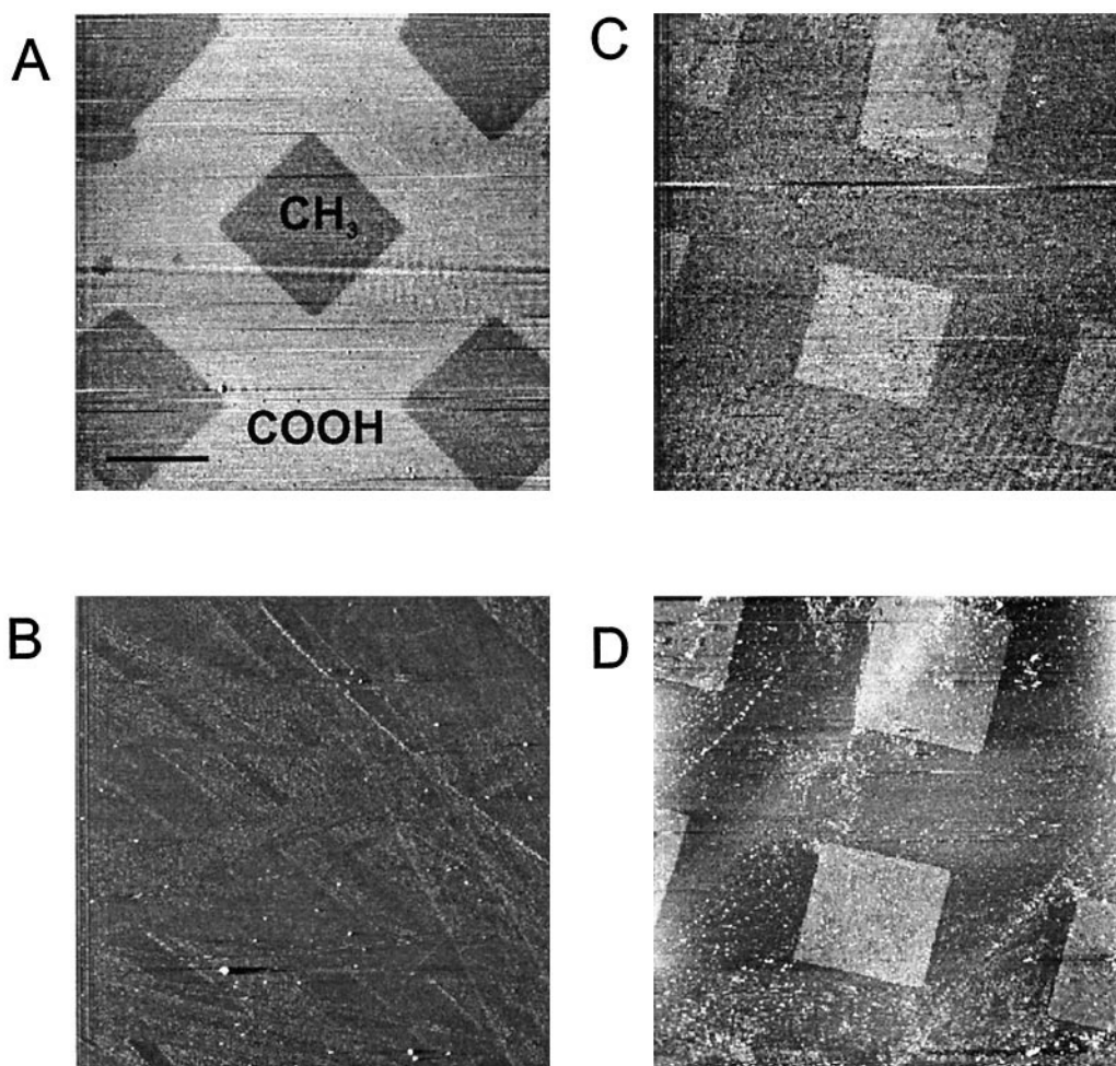
FIGURE 4 Scanning force microscopy images in the lateral force mode, indicating the interaction between the tip and the surface ( A and C ) and topography mode, indicating the height of the sample ( B and D ). ( A and B ) The clean, chemically patterned surface of hydrophobic methyl 20 \times 20 \mu\text{m}^2 squares in an environment of hydrophilic carboxylate groups. ( C and D ) The surface after overnight incubation in a solution of 10 \mu\text{g/ml} SC3 at pH 7, followed by heating the surface in 2% SDS for 10 min at 100^\circ\text{C} . The lateral force mode measurements were performed with a Topometrix Discoverer (TMX2010) atomic force microscope with a closed liquid cell. All measurements were performed in ethanol. High lateral force and raised topological surfaces are indicated by the lighter color. The bar represents 20 \mu\text{m} .
